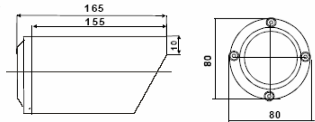
External dimensions unit: mm
